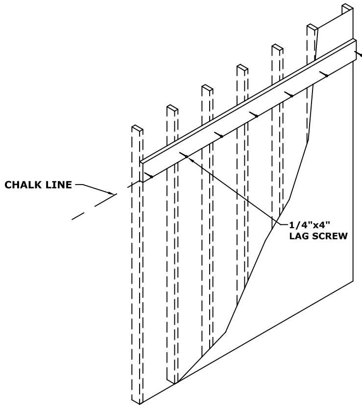
Wall Attachment w/ Ledger Board
